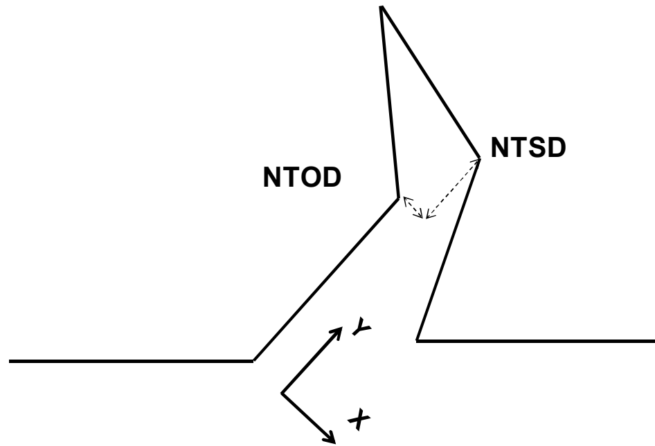
Figure 6-16. Fracture Parameters Determined: (NTOD and NTSD)
