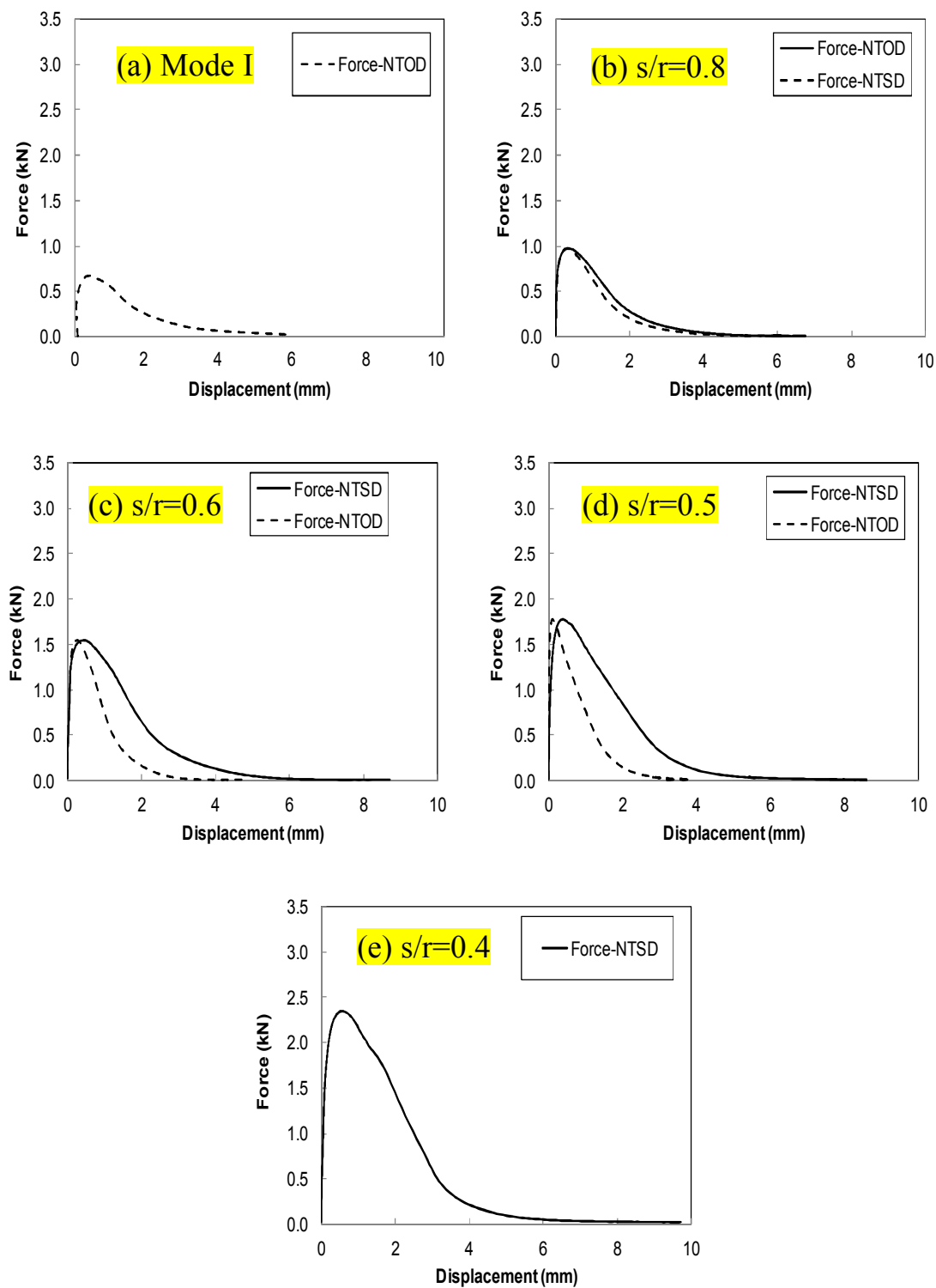
Figure 6-19. Force-NTOD and Force-NTSD Curves ( 50^\circ inclined notch)
