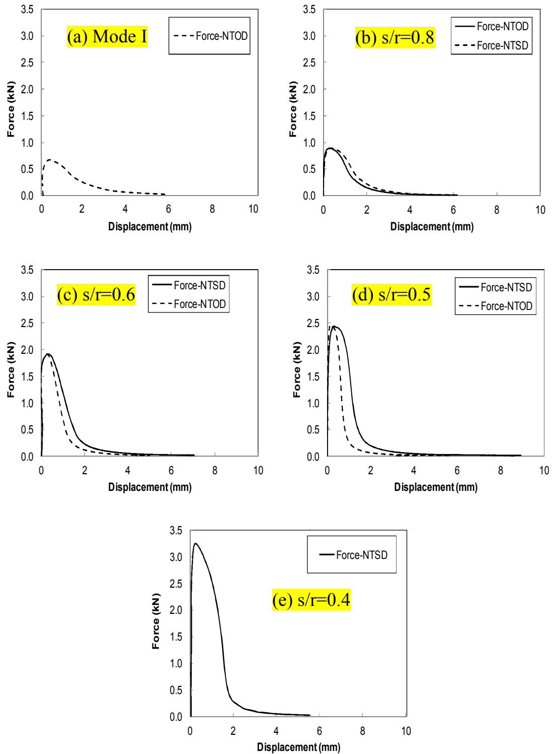
Figure 6-18. Force-NTOD and Force-NTSD Curves ( 45^\circ inclined notch)
